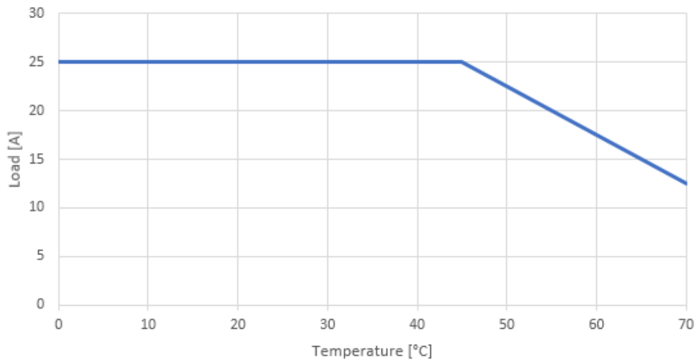
Total output current - Derating @ 24V DC
